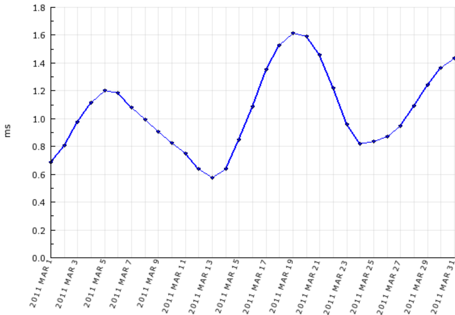
Excess of the length of day
